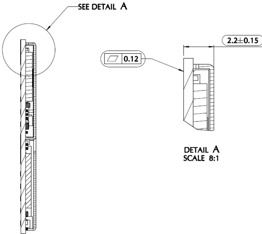
Figure 26: LE910C1-SV Mechanical Dimensions (Side view)
