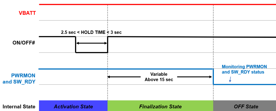
Figure 7: Hardware Shutdown
